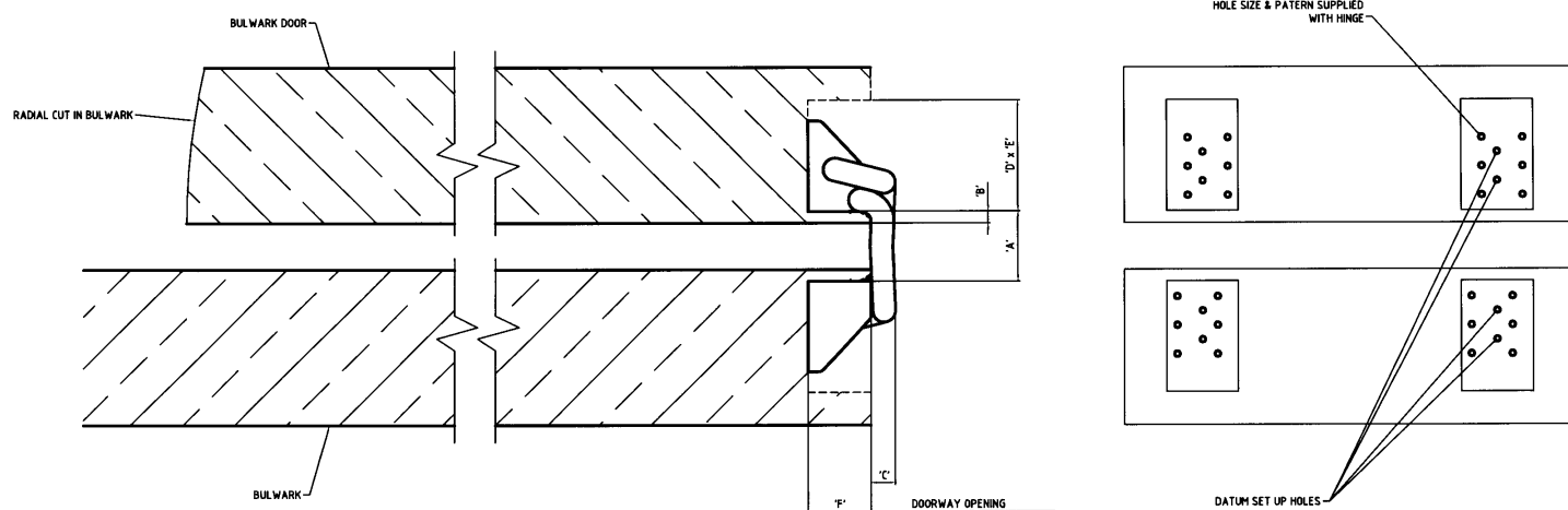
PLAN VIEW OF BULWARK DOOR 180° OPEN - VERTICAL HINGING
